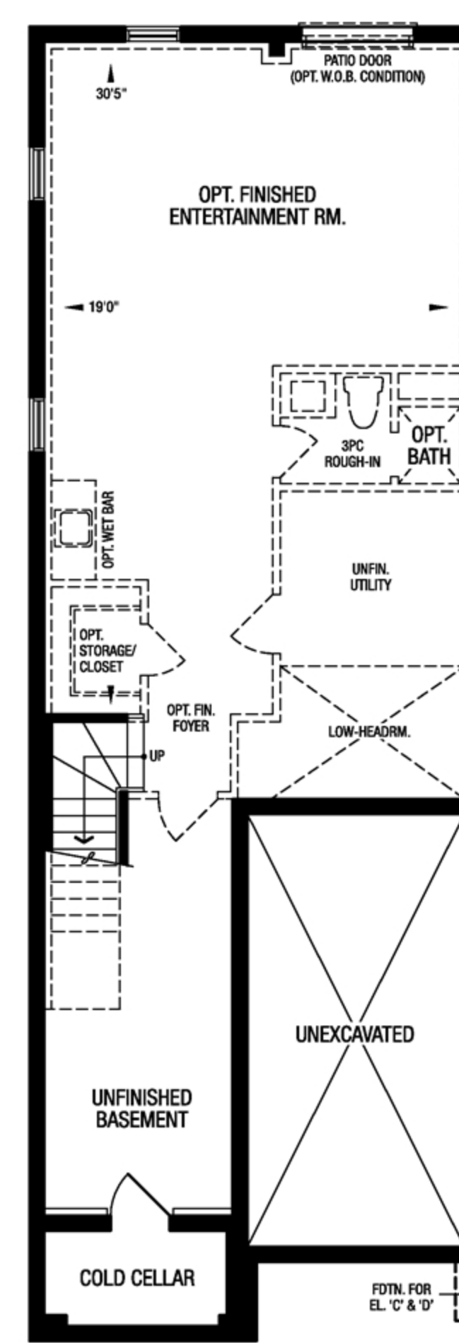
BASEMENT ELEV. A, B, C & D
