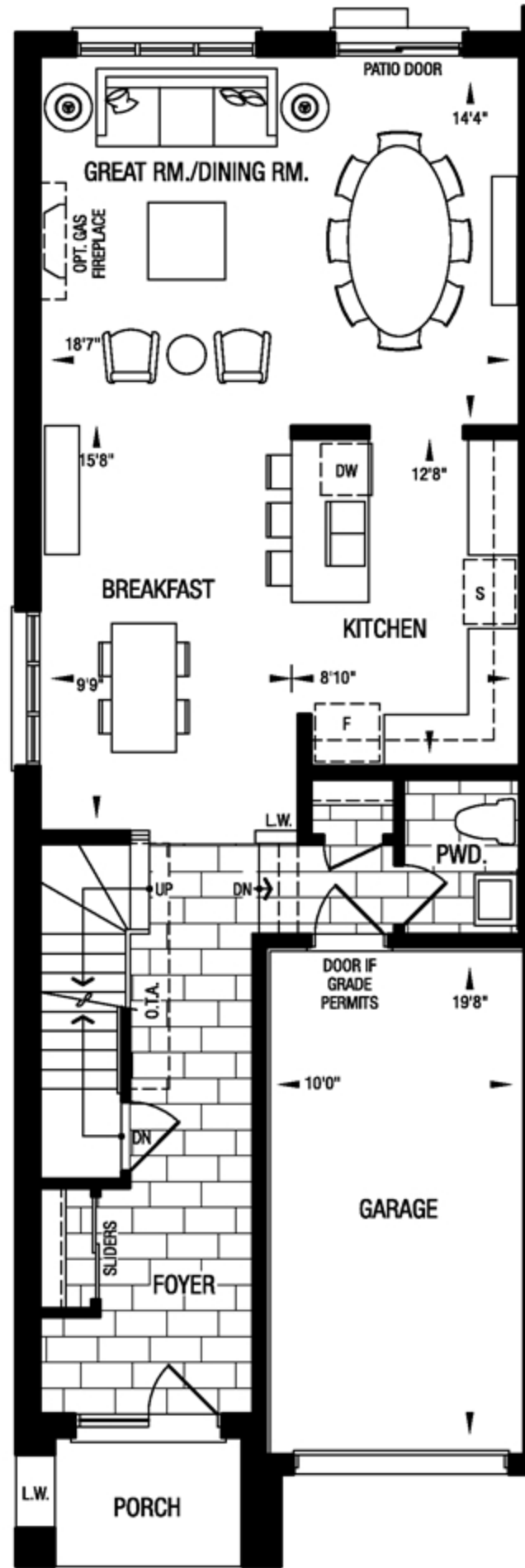
GROUND FLOOR ELEV. A & B
