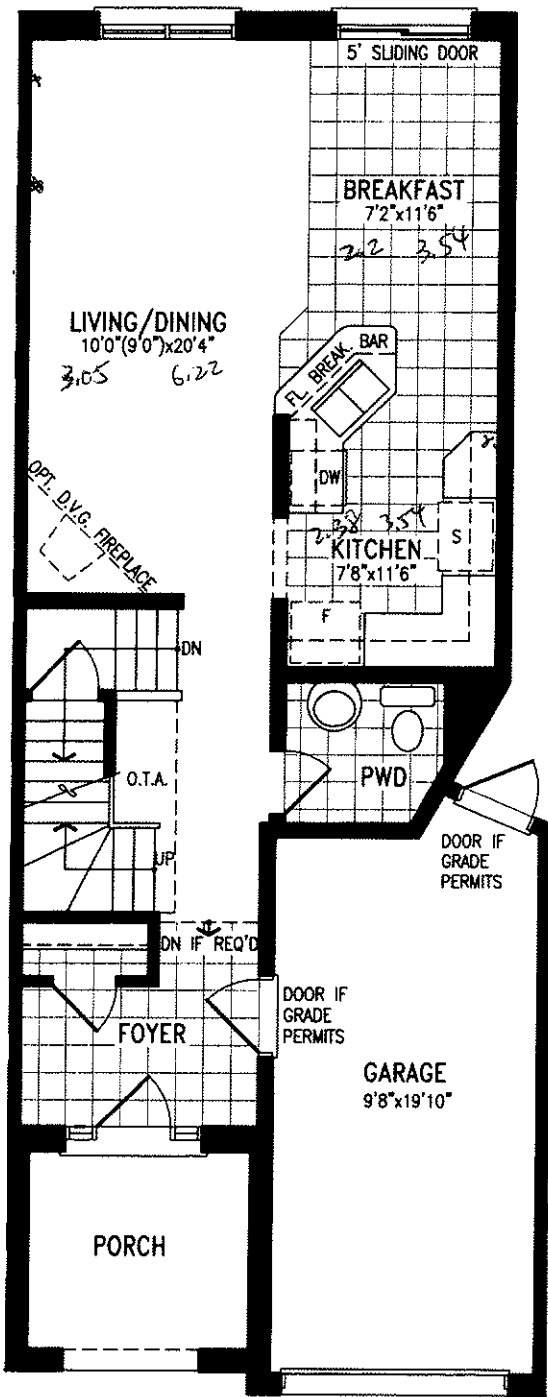
Elevation A & B GROUND FLOOR
